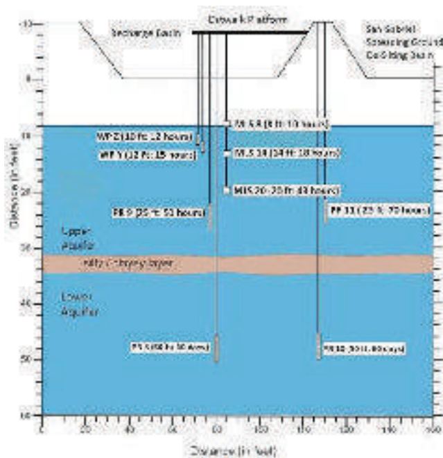
Instrumentation of groundwater recharge test basin associated with monitoring data provided in table below.
